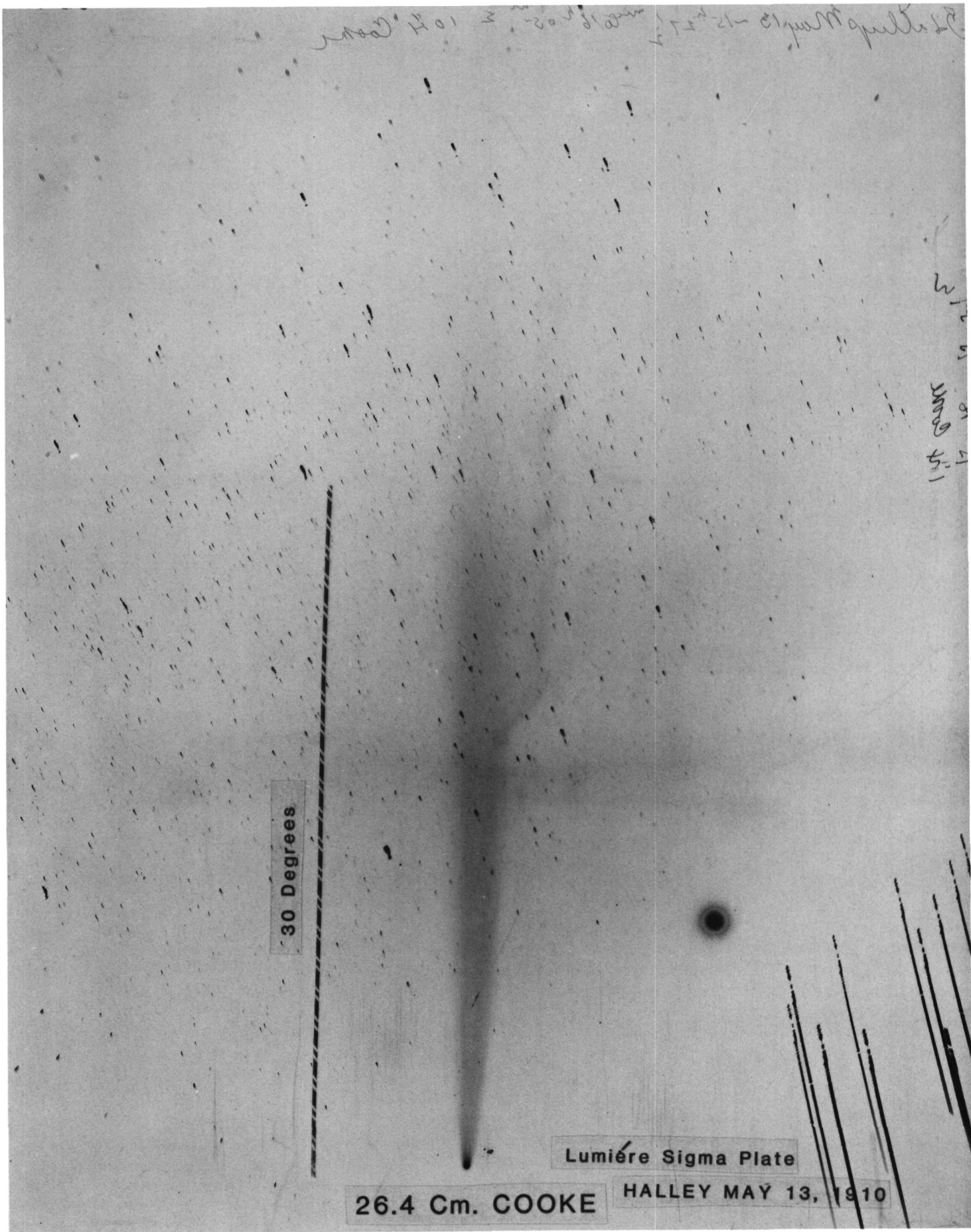
Figure 6. Photograph of Comet Halley obtained on May 13, 1910.
